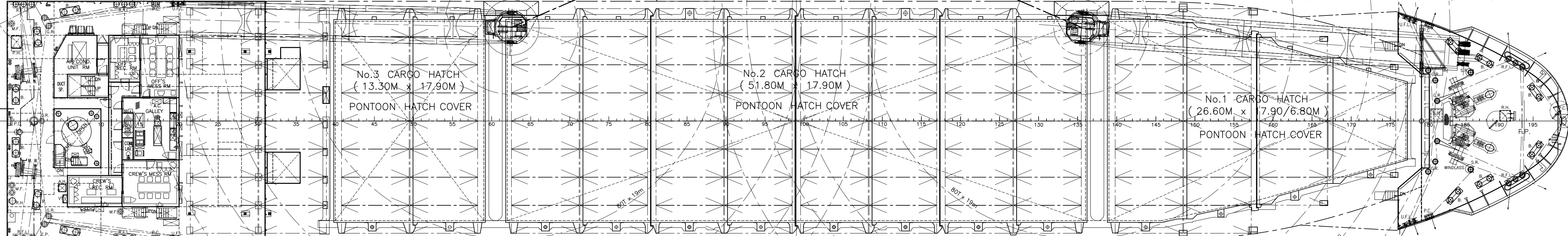
F'CLE DECK
