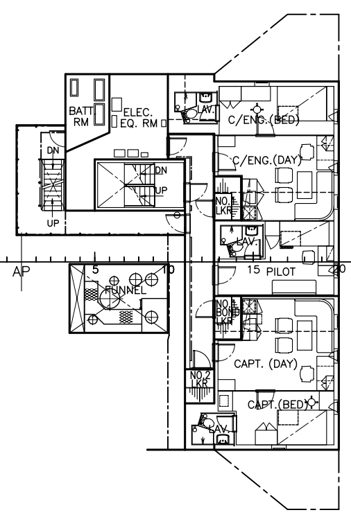
A - DECK
