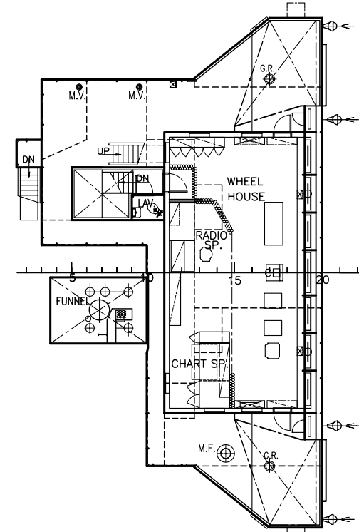
D - DECK
