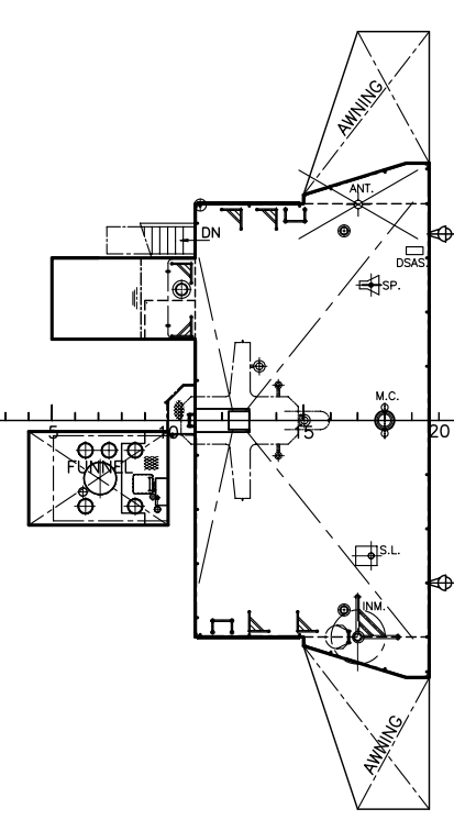
C - DECK
